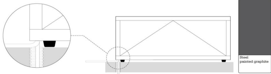
Universal vertical cable output with rubber-feet (suitable for both indoor and outdoor)
